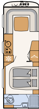
650 RQT 4 sleeping berths
