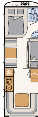
730 FKR 8 sleeping berths
