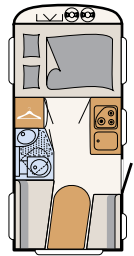
415 QL 3 sleeping berths
